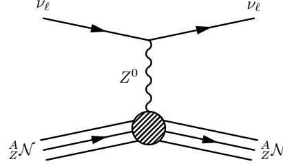
FIGURE 1: Feynman diagram for CE \nu NS in the SM. Details are in the text.
